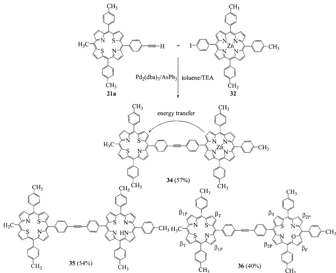
Scheme 6. Synthesis of unsymmetrical covalent dimer 34 and the structures of dimers 35 and 36 .
