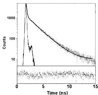
Figure 4. Fluorescence decay profile and the weighted residuals distribution fit of dimer 34 . The excitation wavelength used was 406 nm and emission was detected at 600 nm.
