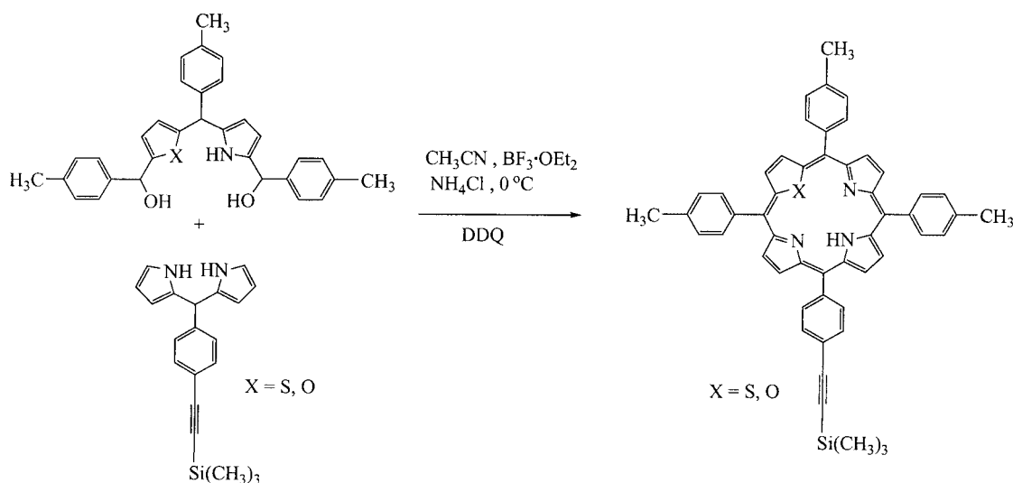
Scheme 1. Synthetic scheme of Lindsey and co-workers for the preparation of monofunctionalised 21-thia- and 21-oxaporphyrins.
