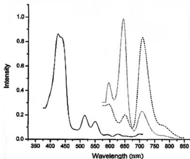
Figure 3. Comparison of emission spectra of dimer 34 (---) and a 1:1 mixture of 21a and 32 (····) recorded at an excitation wavelength of 550 nm in toluene. The excitation spectrum of dimer 34 ( \circ ) recorded at an emission wavelength of 750 nm is also shown.
