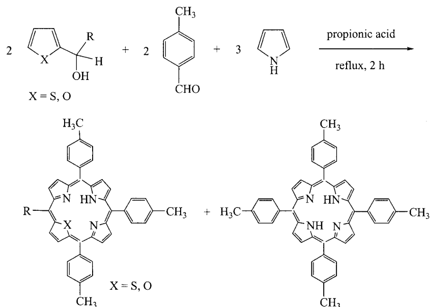
Scheme 2. Mono-ol method for the synthesis of monofunctionalised 21-thia- and 21-oxaporphyrins.
