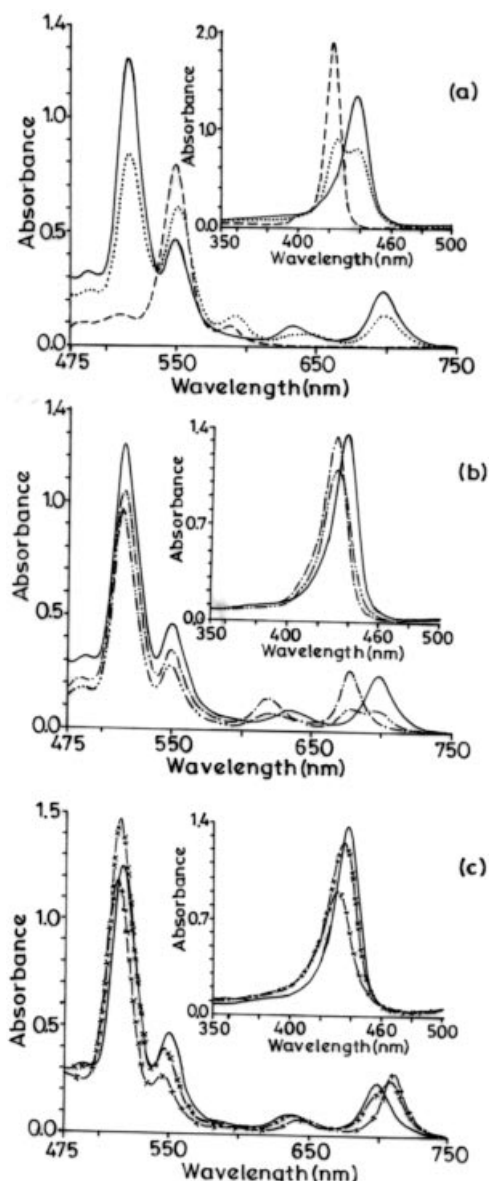
Figure 2. Q-band absorption spectra of: (a) 21a ( \circ ), 32 (---), 34 (····); (b) 21a ( \circ ), 33 (-·-·-), 35 (- - - -); (c) 21a ( \circ ), 29 (-·-·-), 36 (- - - -) recorded in toluene. Their corresponding Soret band absorption spectra are shown in the insets. The concentrations used for Q-band spectra was 5 \times 10^{-5} M and for Soret band was 5 \times 10^{-6} M.
