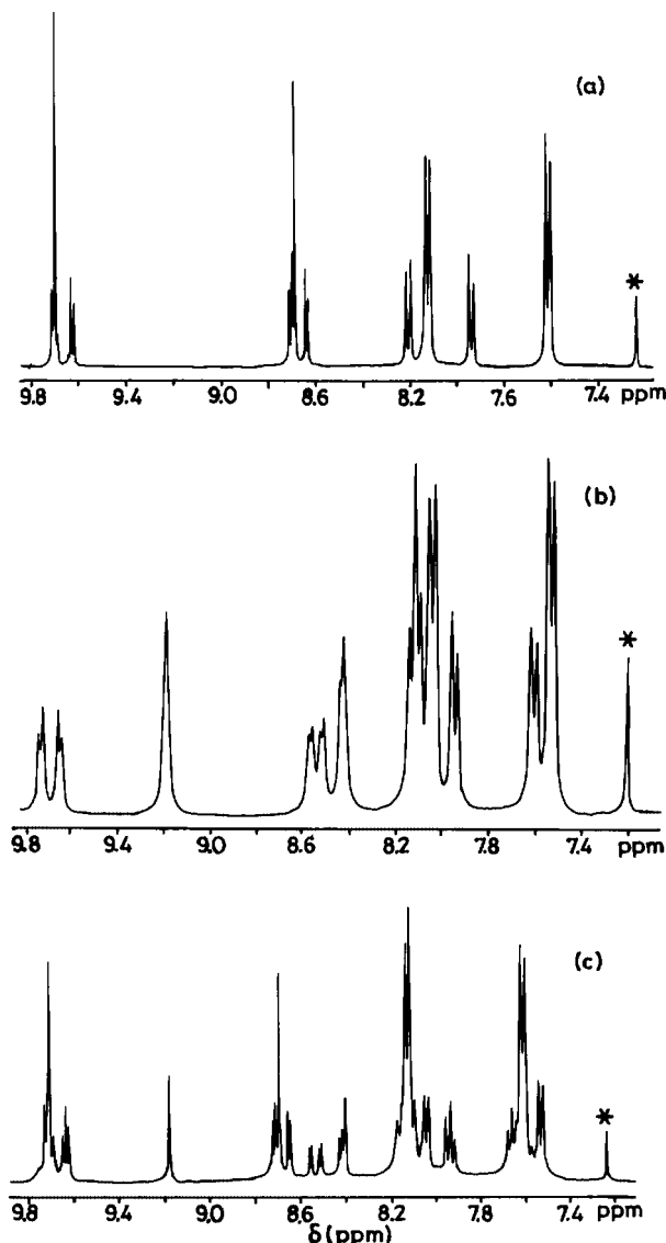
Figure 1. ^1\text{H} NMR spectra of 21a (a) 29 (b) and 36 (c) recorded in \text{CDCl}_3 .
