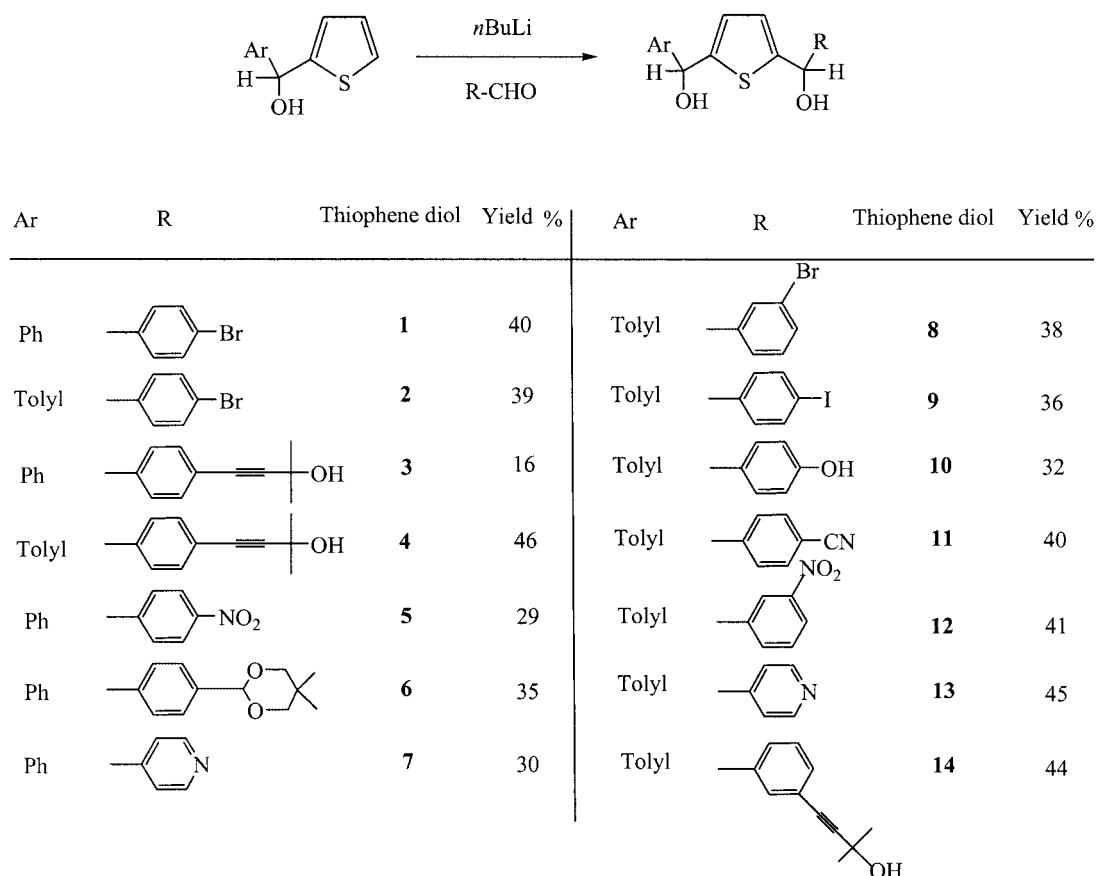
Scheme 4. Synthesis of unsymmetrical thiophene diols 1–14 .
