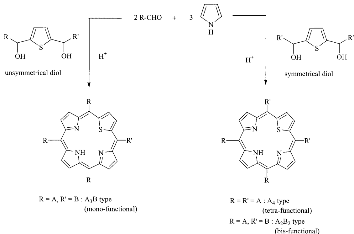
Scheme 3. Symmetrical and unsymmetrical thiophene diol methods for the preparation of functionalised 21-thiaporphyrins.
